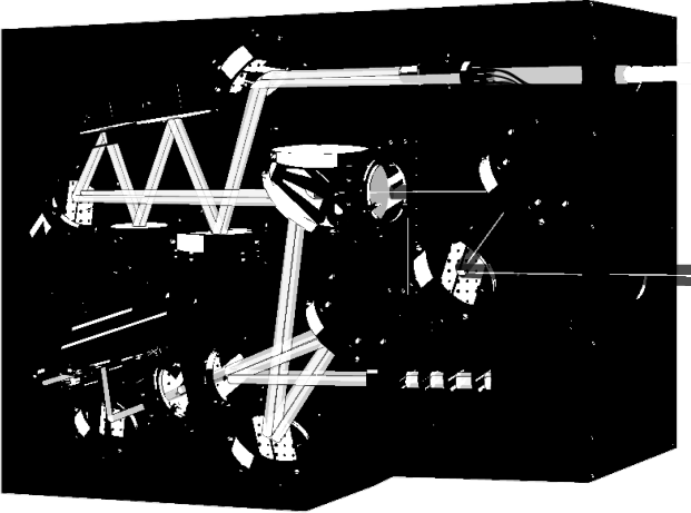
Figure 3. View of the AO optical bench, CANOPUS
