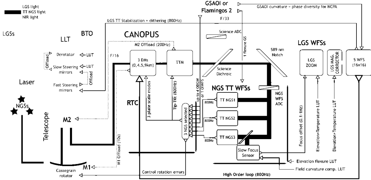
Figure 2. GeMS “synaptic” diagram, showing major subsystems and their relationship, all loops and offloads.
