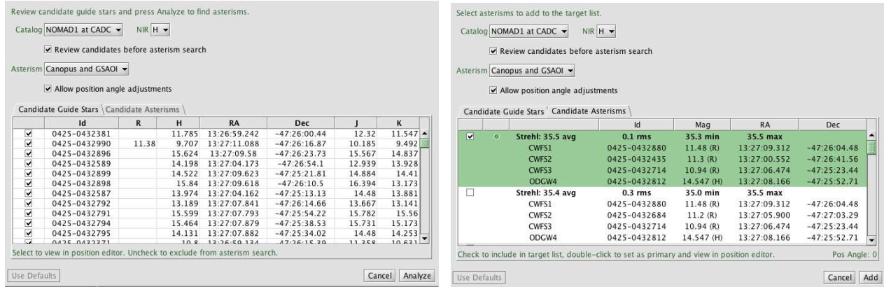
Figure 9. GeMS guide star search window. The left panel shows the list of potential stars used by MASCOT to search for the best asterism. The right panel shows the result of the search. The best asterism is highlighted in green. The user has the option to select one or more asterisms from the candidate list and add them to the target component.
