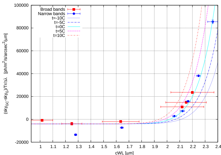
Figure 7. Difference in the background signal between the data obtained with the configuration GSAOI+CANOPUS and with GSAOI only in units of \text{ph/s/arcsec}^2/\mu\text{m}/\text{m}^2 . The lines represent the thermal emission from a black body (see the text).
