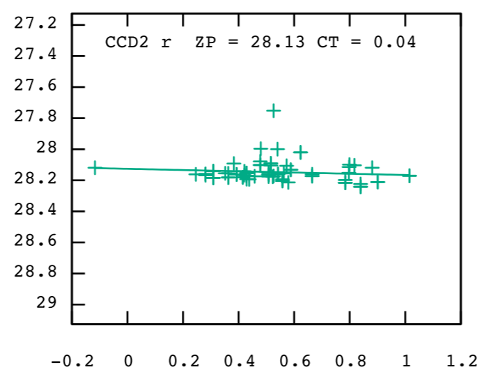
(g-r)
