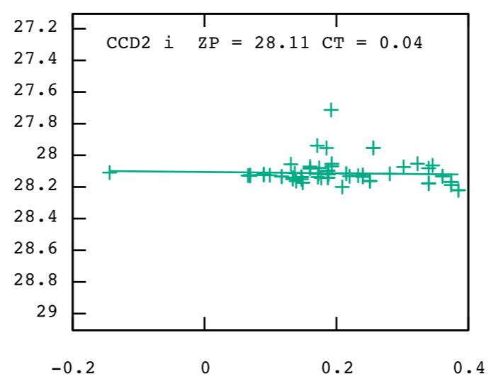
(r-i)
