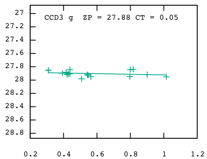
(g-r)
