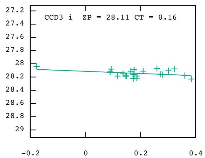
(r-i)
