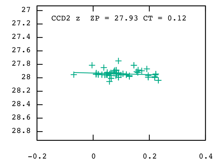
(i-z)
