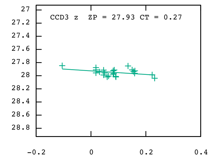
(i-z)
