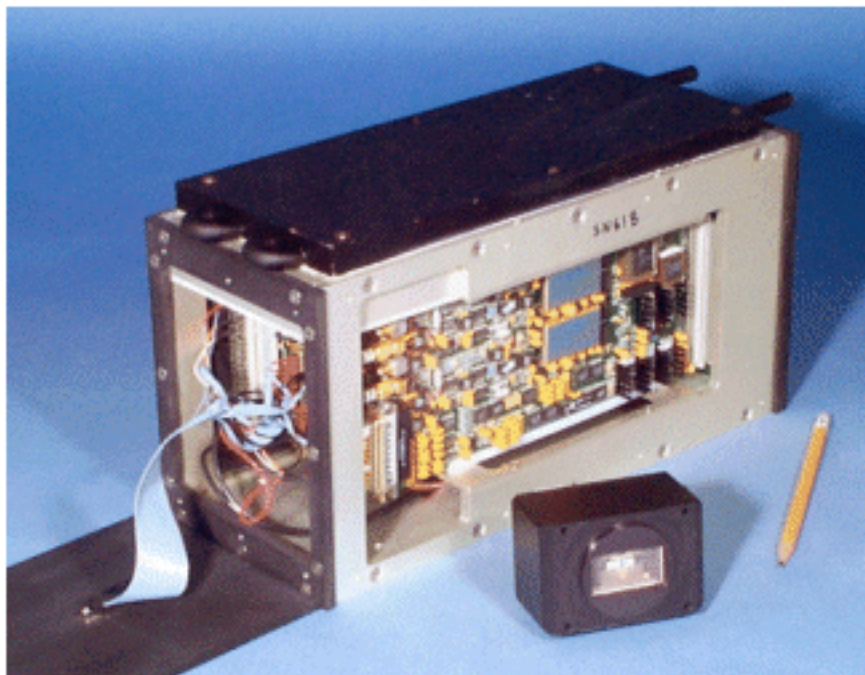
Figure 13. WFS Controller and CCD Housing.
