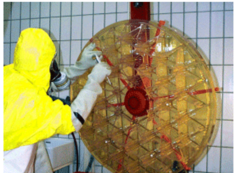
Figure 4. Secondary mirror at Zeiss.
