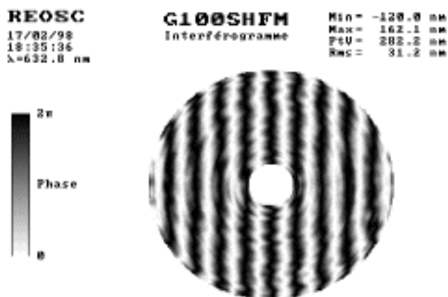
Figure 1. REOSC measuring results for Primary Mirror #1.
