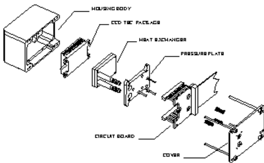
Figure 12. WFS CCD housing.
