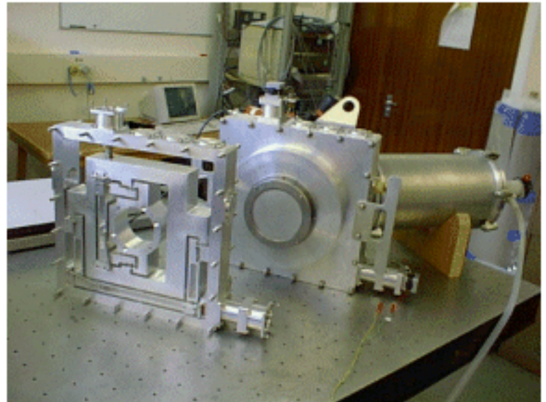
Figure 16. x,y,z CCD Translation Stage
