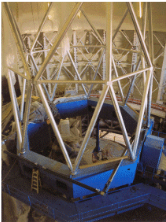
Figure 2. Installation of the northern telescope structure.
