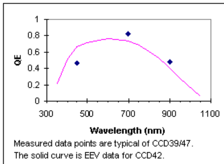
Figure 11. CCD39/47 Quantum Efficiency.
