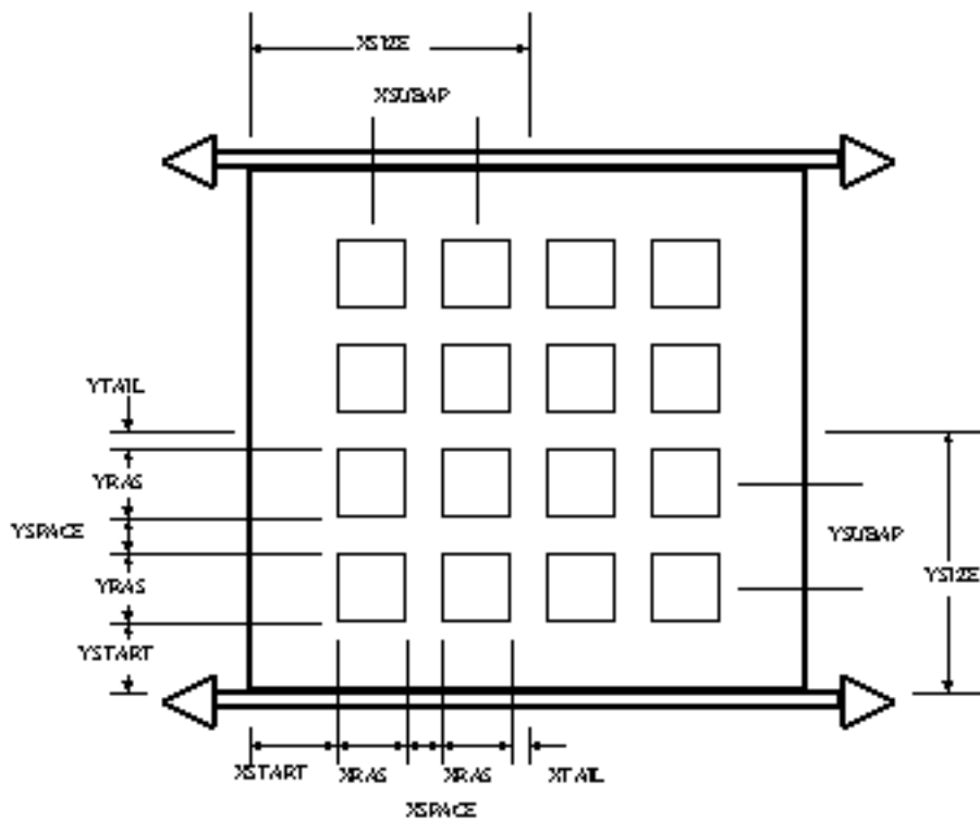
Figure 14. Generalized Readout Geometry
