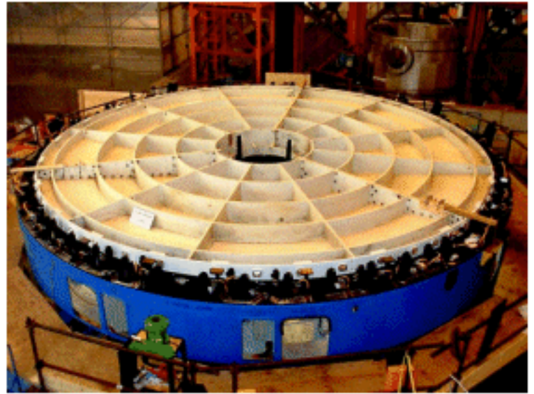
Figure 3. The first primary mirror cell with steel dummy mirror in place.
