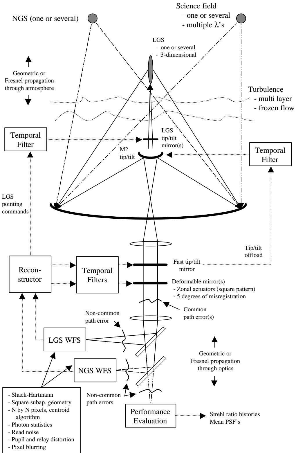
Figure 1: Simulation Features
