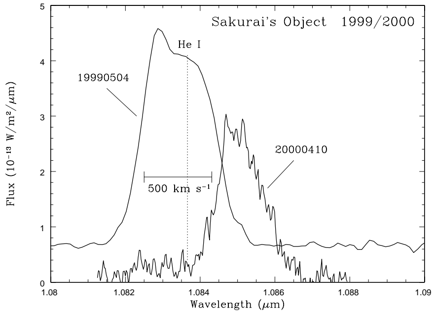
Figure 8. Helium line profiles in 1999 and 2000. The resolution of the 1999 spectrum is 60 \text{ km s}^{-1} ; that of the 2000 spectrum, which has been slightly smoothed, is 19 \text{ km s}^{-1} . The small fluctuations in the latter are due to noise.
