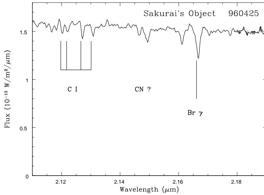
Figure 2. A portion of the K band spectrum of 1996. Vertical lines denote laboratory wavelengths of identified lines.
