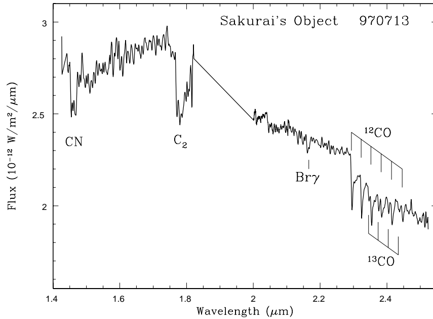
Figure 3. 1.4-2.5 \mu\text{m} spectrum in 1997. Vertical lines for CO are at the wavelengths of band heads.
