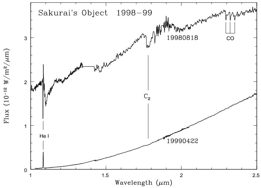
Figure 7. Comparison of 1-2.5 \mu\text{m} spectra in late 1998 and early 1999.
