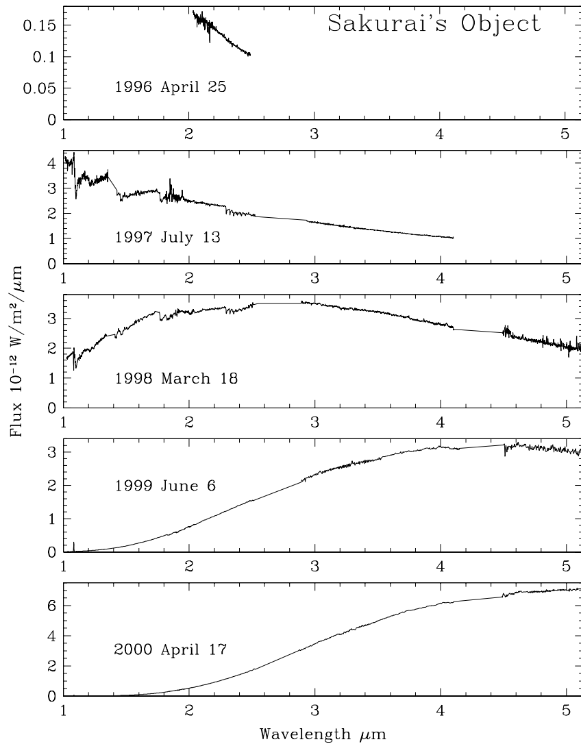
Figure 1. UKIRT/CGS4 spectra of Sakurai's Object from 1996 to 2000. The spectra are interpolated in the gaps at 1.35-1.42 \mu\text{m} , 2.5-2.9 \mu\text{m} , and 4.1-4.5 \mu\text{m} .
