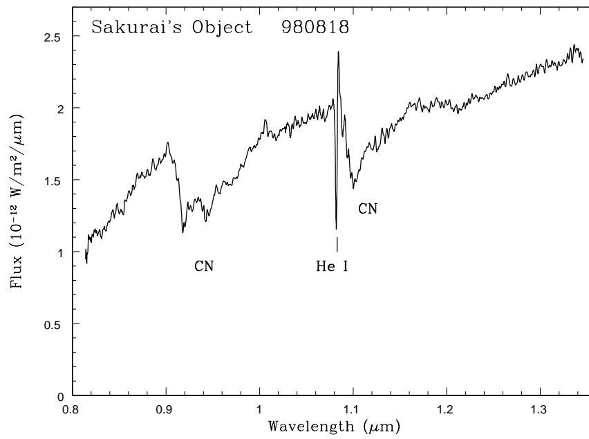
Figure 4. UKIRT/CGS4 I-J band spectrum in 1998
