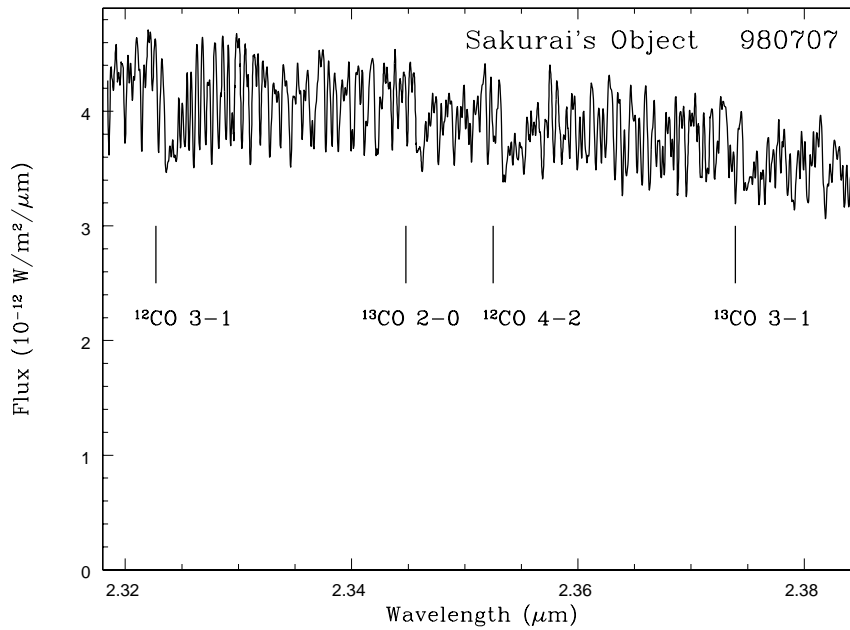
Figure 6. High resolution spectra of a portion of the CO first overtone band. The laboratory wavelengths of band heads of ^{12}\text{CO} and ^{13}\text{CO} are indicated and the heads are redshifted by roughly 0.002 \mu\text{m} .
