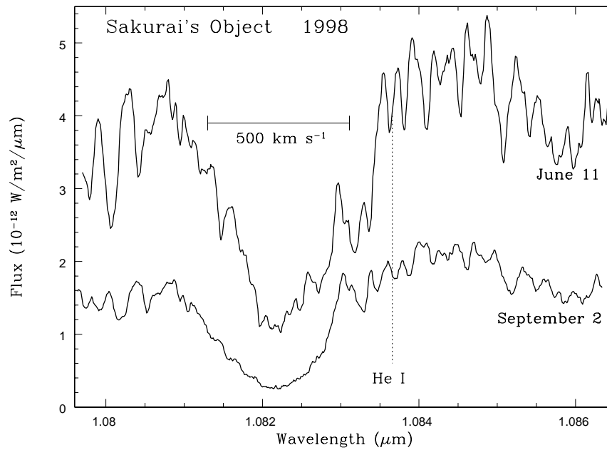
Figure 5. UKIRT/CGS4 high resolution spectra of the He I 1.083 \mu\text{m} line in 1998. the dashed vertical line corresponds to the wavelength of the helium line at the radial velocity of Sakurai's Object as observed on June 11
